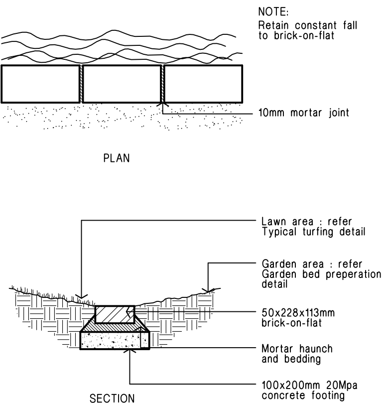
Brick garden edge Detail.
