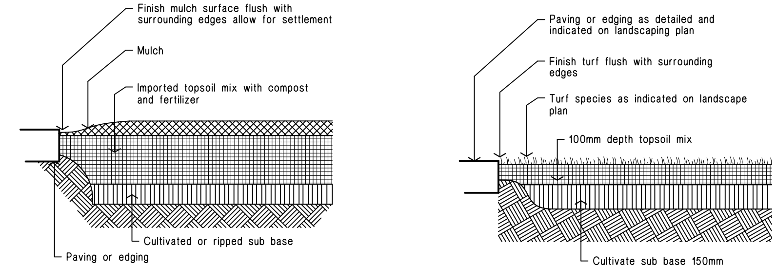
Ground preparation Planting area using imported topsoil Detail. Not.To.Scale.
