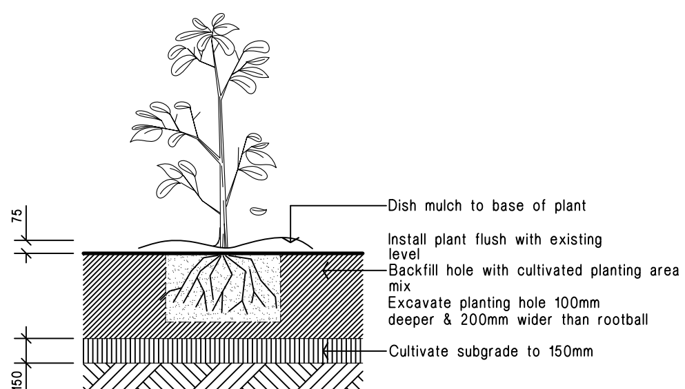
Planting in garden beds Detail. Not.To.Scale.
